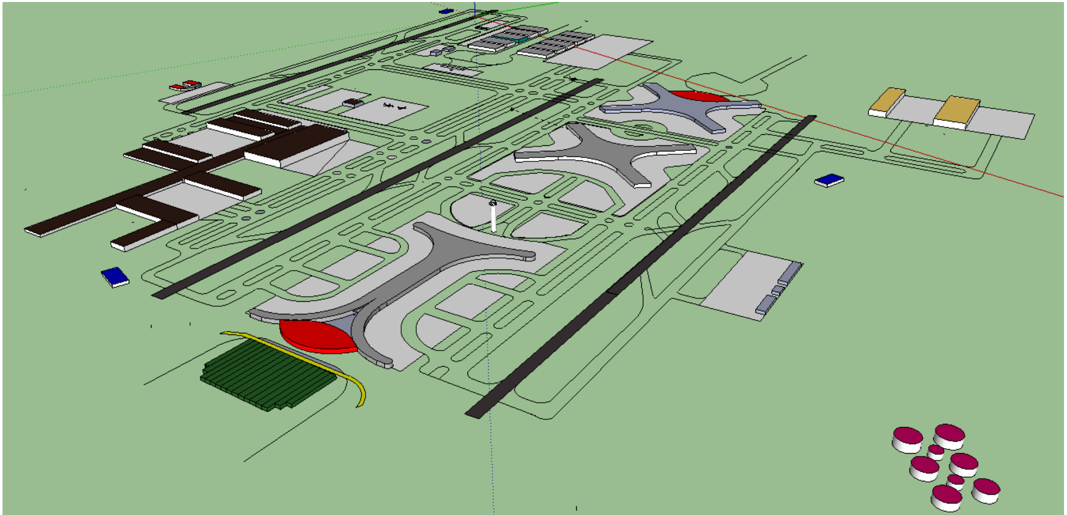
Land use plan of Jeddah Airport, 3D
