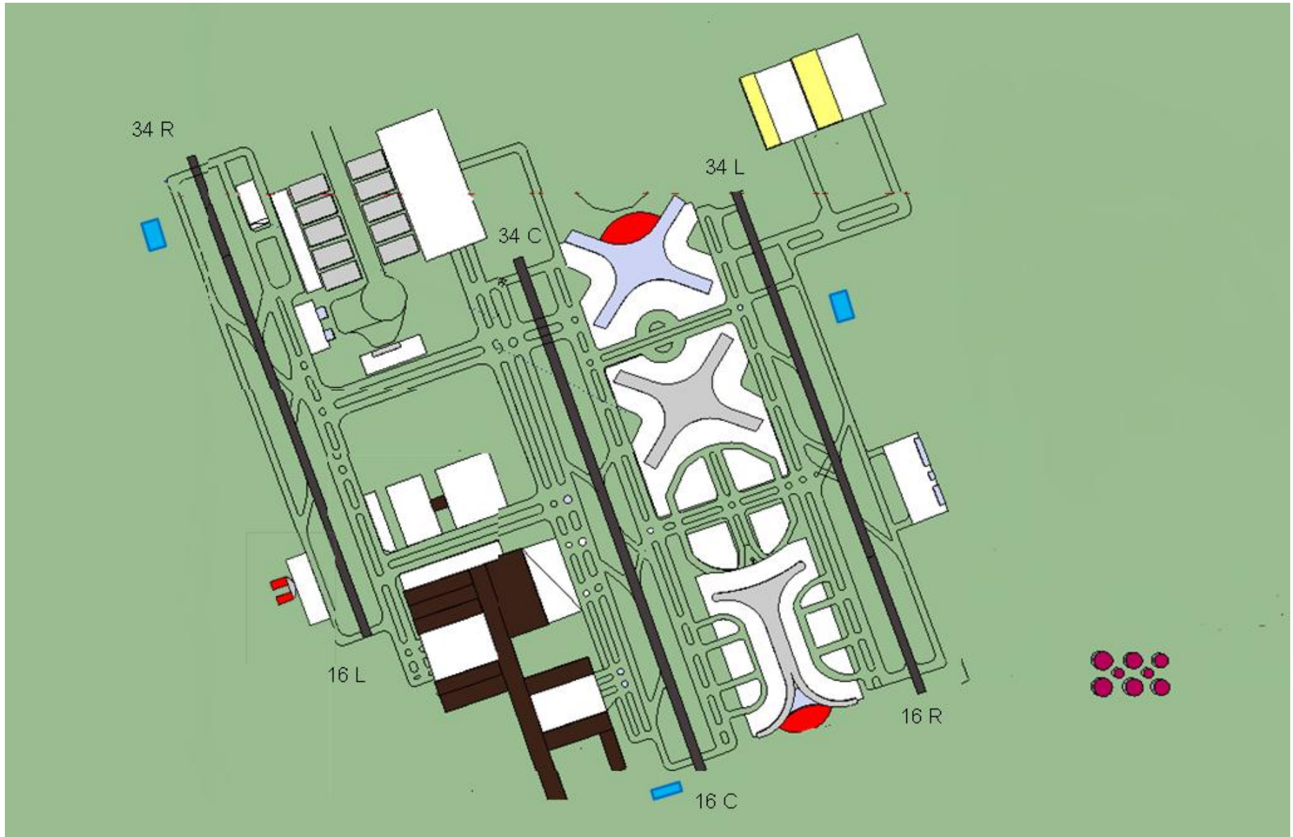
Land use plan of Jeddah Airport, helicopter view
